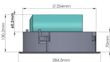
With Sonos ERA100 Speaker
