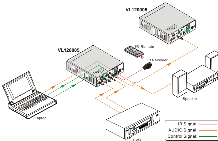
Figure 3- 1 System Diagram
