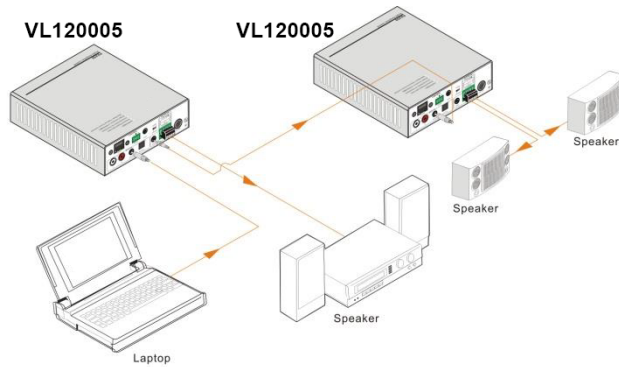
Figure 3- 4 Loop Connection
