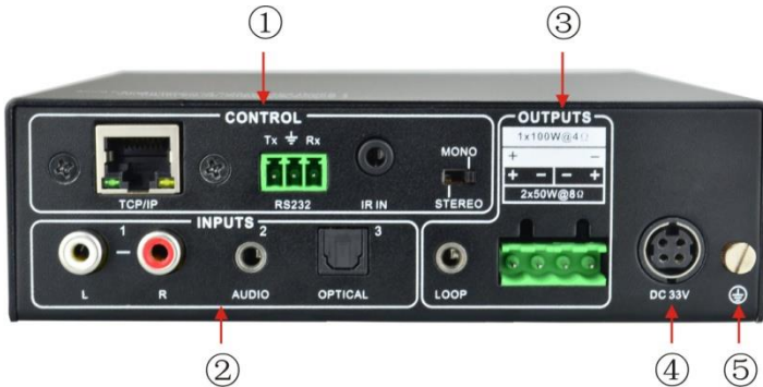
Figure 2- 2 Rear Panel of VL120005
