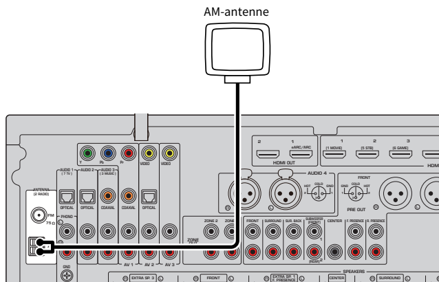
Enheden (bagside)
