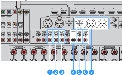
Enheden (bagside)
