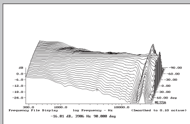
Fig.5 Klipsch RP-600M, lateral response family at 50", normalized to response on tweeter axis, from back to front: differences in response 90°–5° off axis, reference response, differences in response 5°–0° off axis.
