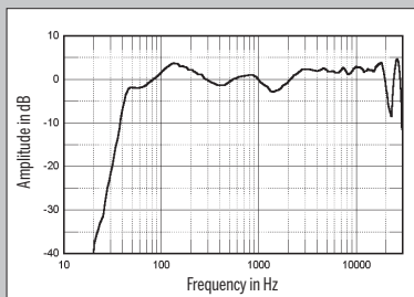
Fig.4 Klipsch RP-600M, anechoic response on tweeter axis at 50", averaged across 30° horizontal window and corrected for microphone response, with complex sum of nearfield woofer and port responses plotted below 300Hz.
