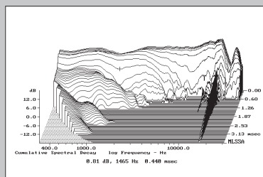
Fig.8 Klipsch RP-600M, cumulative spectral-decay plot on tweeter axis at 50° (0.15ms risetime).
