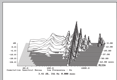
Fig.2 Klipsch RP-600M, cumulative spectral-decay plot calculated from output of accelerometer fastened to center of sidewall (MLS driving voltage to speaker, 7.55V; measurement bandwidth, 2kHz).
