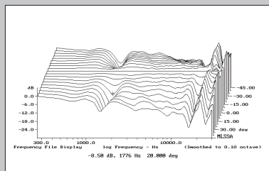
Fig.6 Klipsch RP-600M, vertical response family at 50°, normalized to response on tweeter axis, from back to front: differences in response 45-5° above axis, reference response, differences in response 5-45° below axis.
