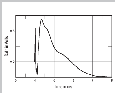
Fig.7 Klipsch RP-600M, step response on tweeter axis at 50° (5ms time window, 30kHz bandwidth).
