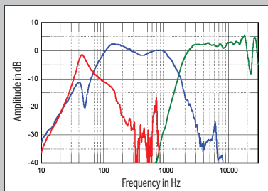
Fig.3 Klipsch RP-600M, acoustic crossover on tweeter axis at 50", corrected for microphone response, with nearfield woofer (blue) and port (red) responses respectively plotted below 350Hz and 750Hz.
