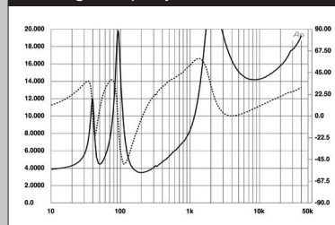
Fig.1 Klipsch RP-600M, electrical impedance (solid) and phase (dashed) (2 ohms/vertical div.).
